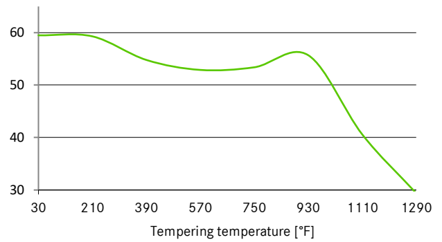
Tempering Chart Hardness HRC
